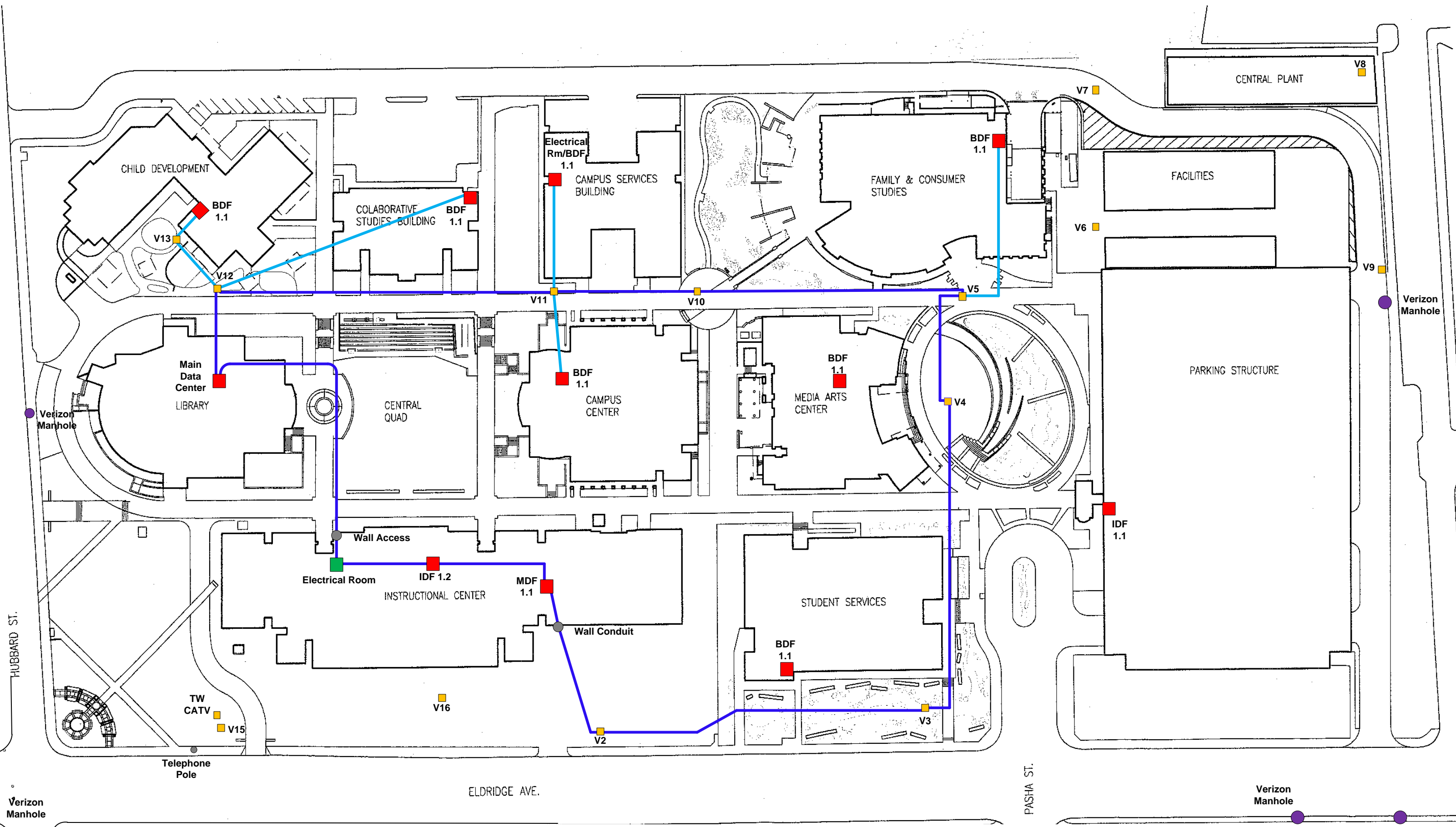
LAMC Fiber Ring Site Plan
